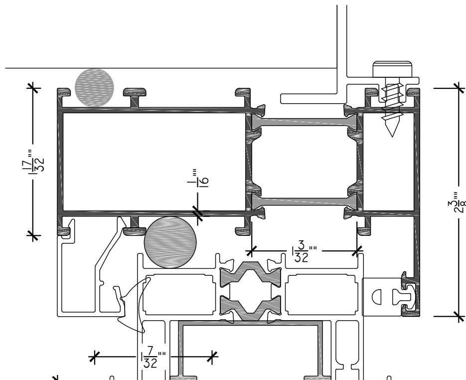
A TRACK DETAIL ARCH REF: NONE SCALE: 1'-0" = 1'-0"
