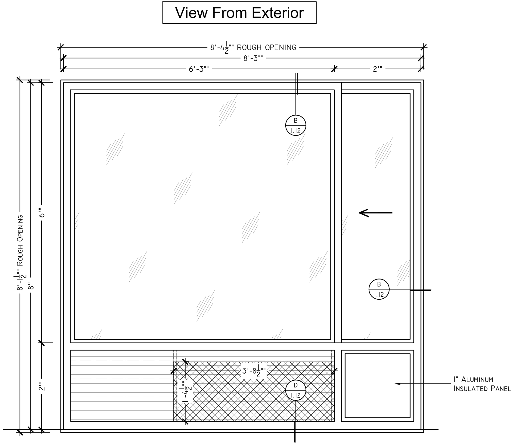
WI SLIDING WINDOW - FIXED/SLIDER ARCH REF: NONE SCALE: 3/4" = 1'-0"
