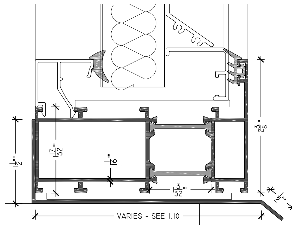
D SILL DETAIL ARCH REF: NONE SCALE: 1'-0" = 1'-0"
