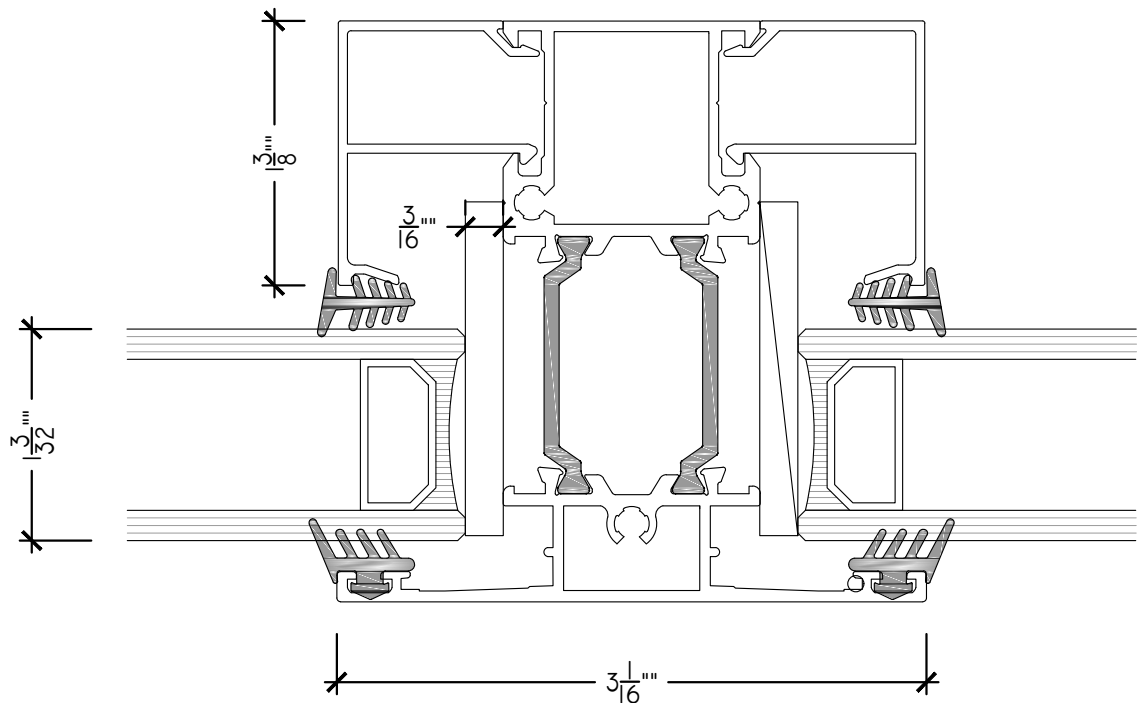
D1 W3 T - PROFILE DETAIL ARCH REF: NONE SCALE: 1'-0" = 1'-0"
