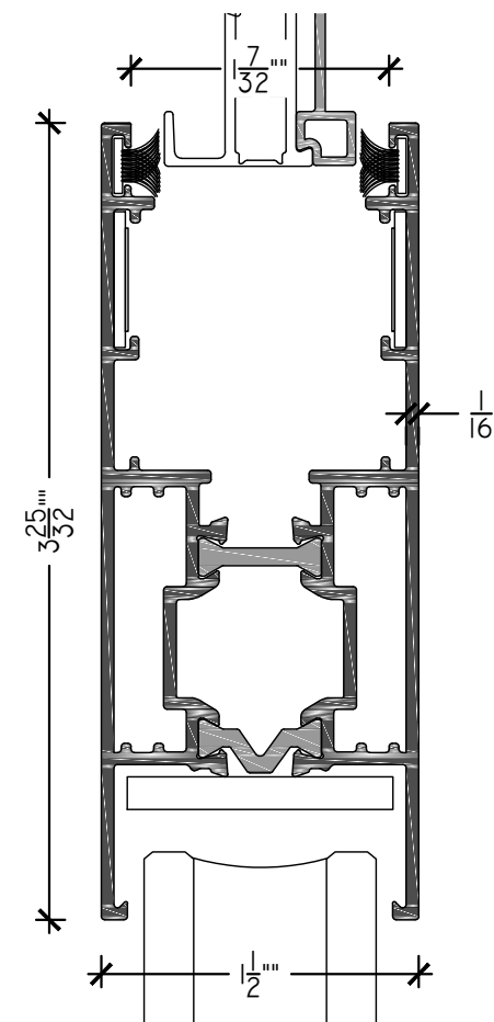
E SLIDER DETAIL ARCH REF: NONE SCALE: 1'-0" = 1'-0"
