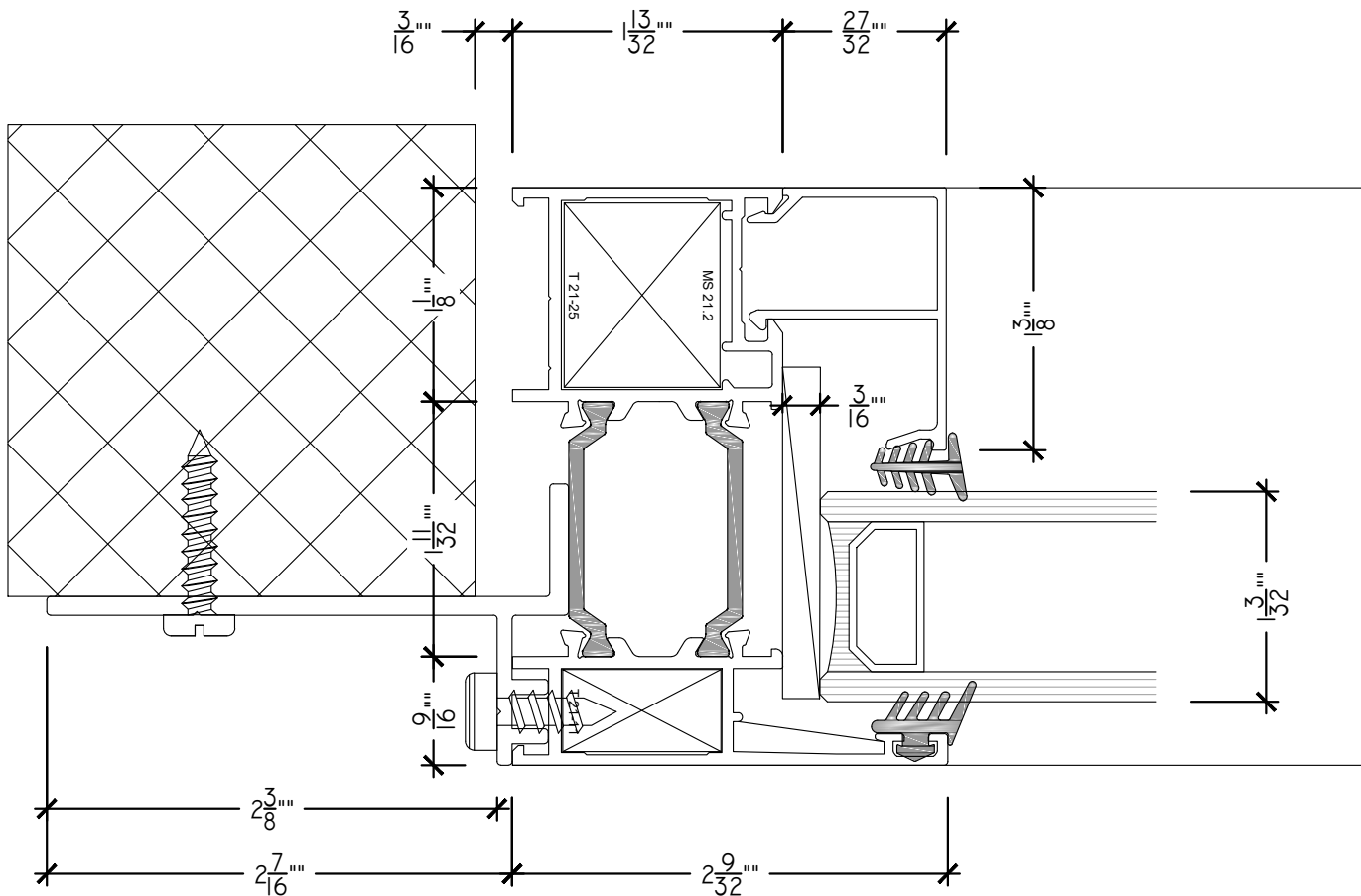
D2 W3 HEAD, JAMB, & SILL DETAIL ARCH REF: NONE SCALE: 1'-0" = 1'-0"
