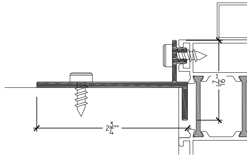
C NAILING FLANGE ARCH REF: NONE SCALE: 1'-0" = 1'-0"
