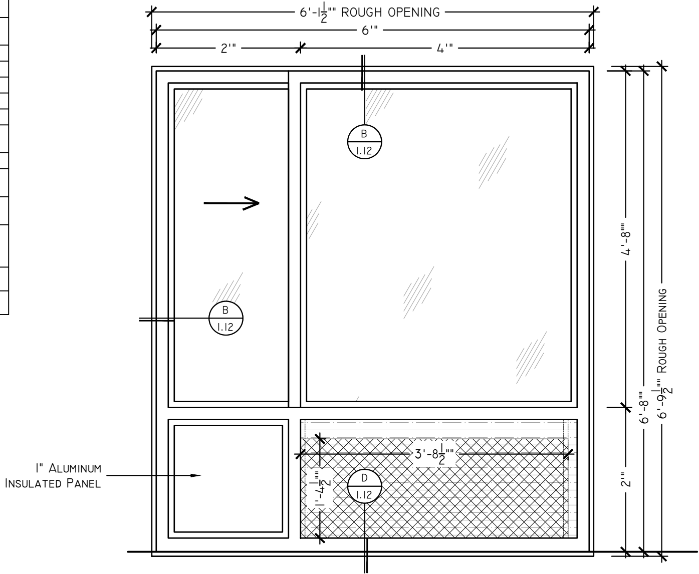
W2 SLIDING WINDOW - SLIDER/FIXED ARCH REF: NONE SCALE: 3/4" = 1'-0"
