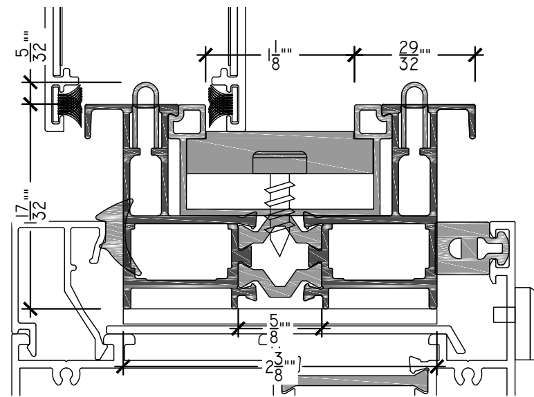
A TRACK DETAIL ARCH REF: NONE SCALE: 1'-0" = 1'-0"
