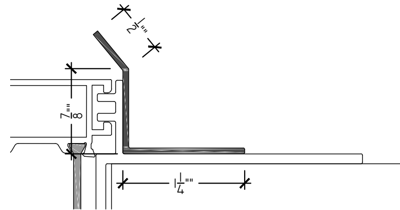
F HEAD FLASHING ARCH REF: NONE SCALE: 1'-0" = 1'-0"
