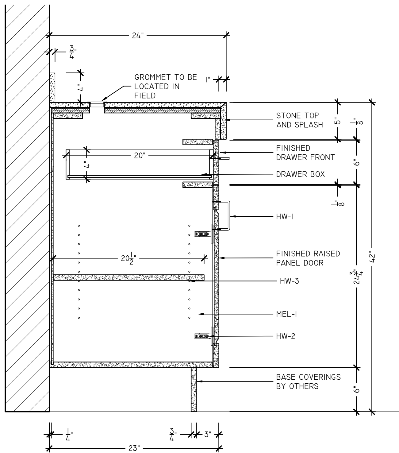
SI SERVER STATION 103 - SECTION SCALE: 1-1/2" = 1'-0" ARCH REF: 3/16/01
