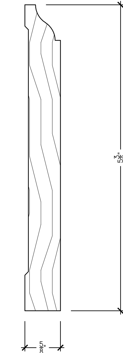
D7 TYPICAL TRIM - DETAIL SCALE: 1'-0\"/>
