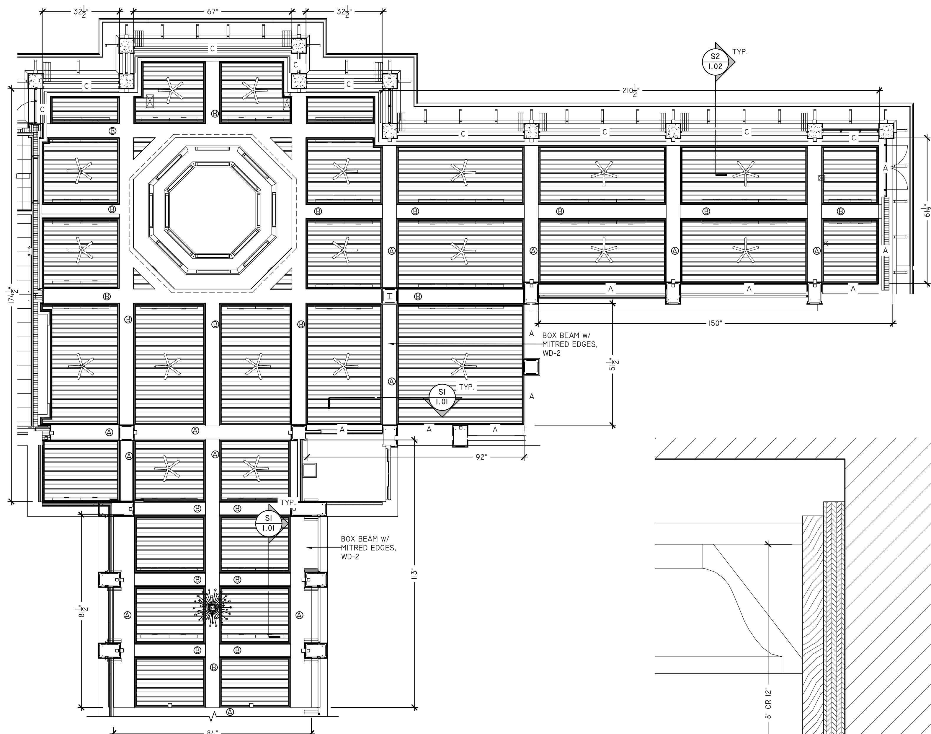
1 BAR 101 - RCP SCALE: NTS ARCH REF: U/A-602
