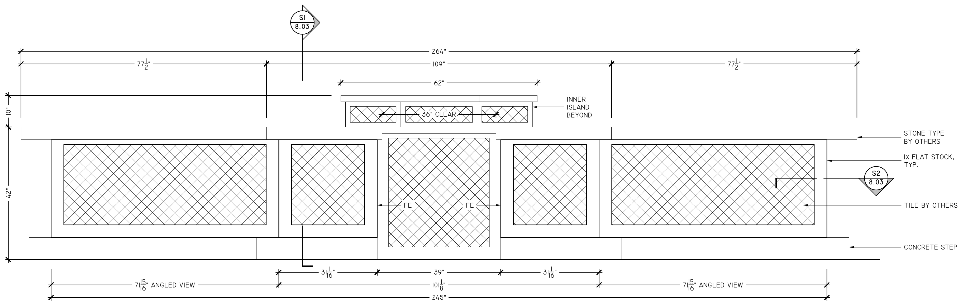
B MAIN BAR - ELEVATION SCALE: 3/4" = 1'-0" ARCH REF: 771-401 (SIP4)
