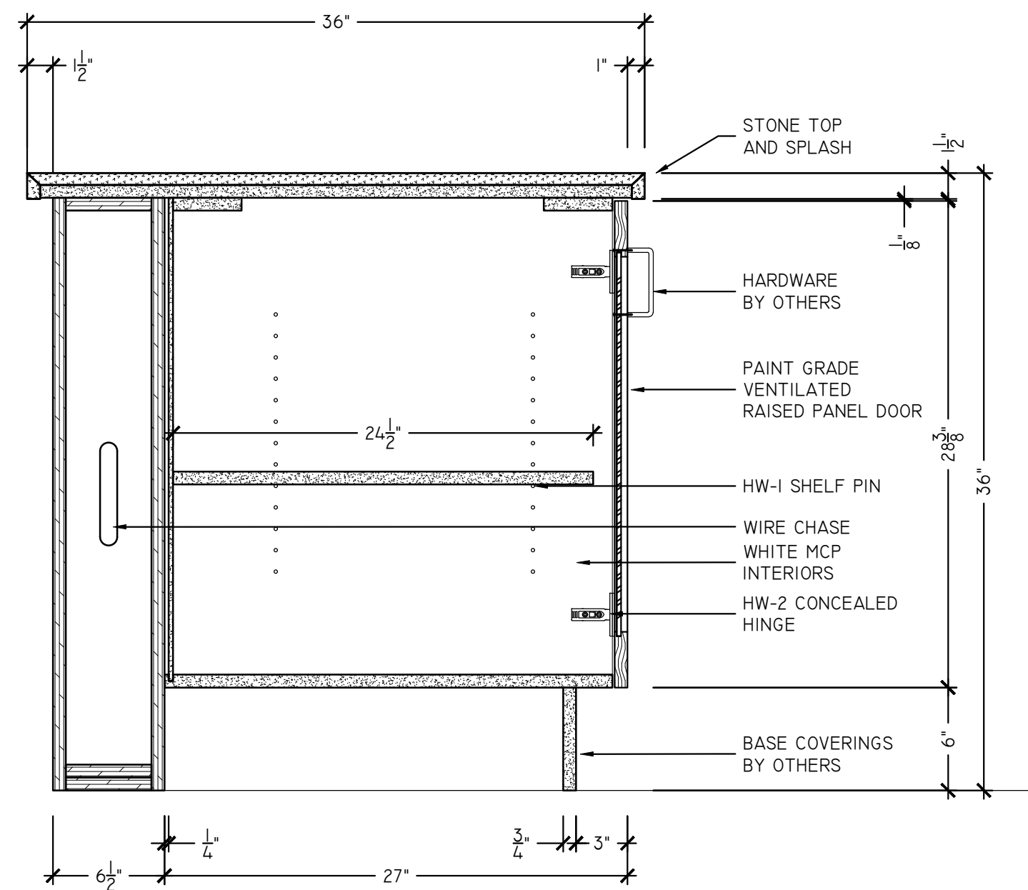
S1 BUFFET III - SECTION SCALE: 1-1/2" = 1'-0" ARCH REF: 6/1101
