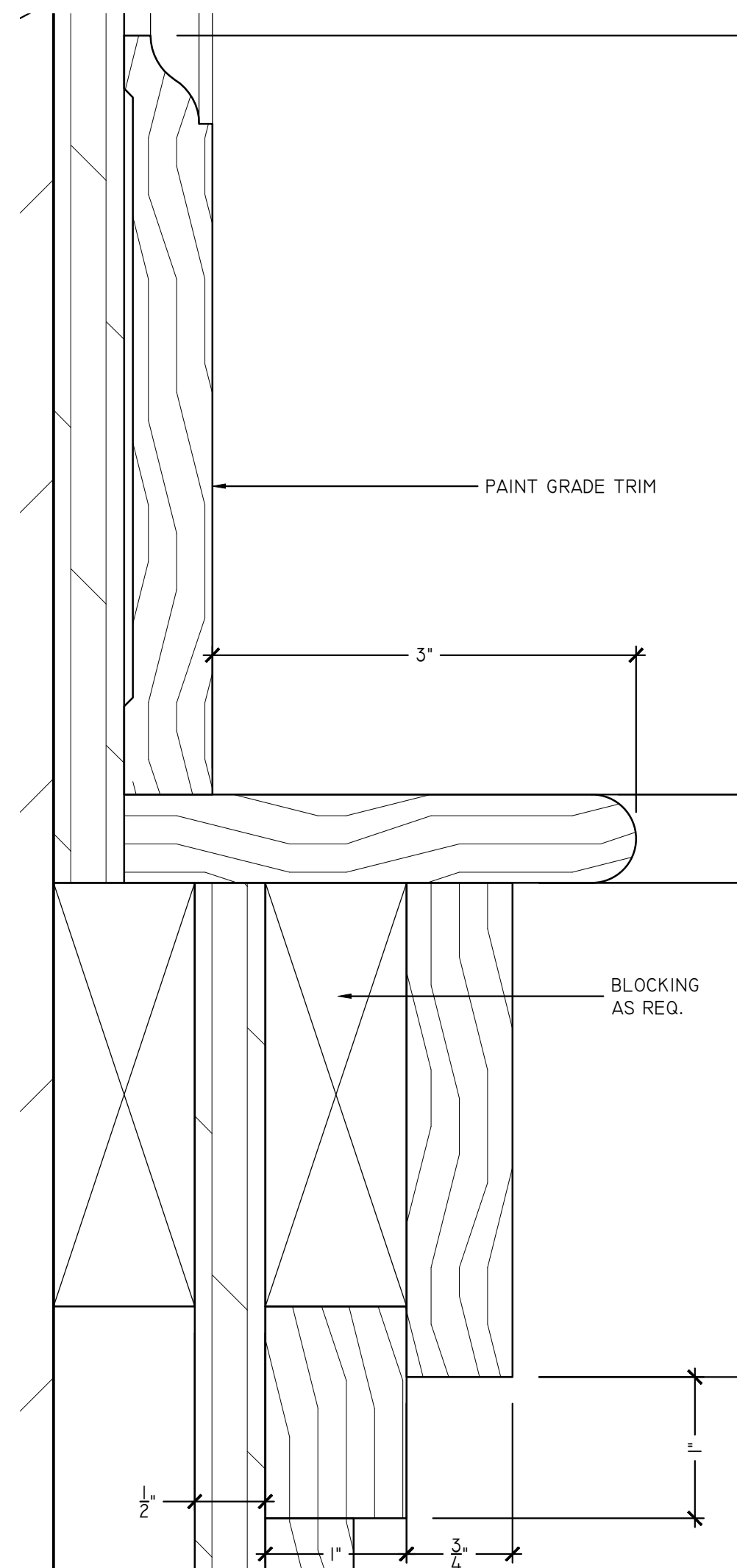
D4 TYPICAL COLUMN - DETAIL SCALE: 1'-0\"/>
