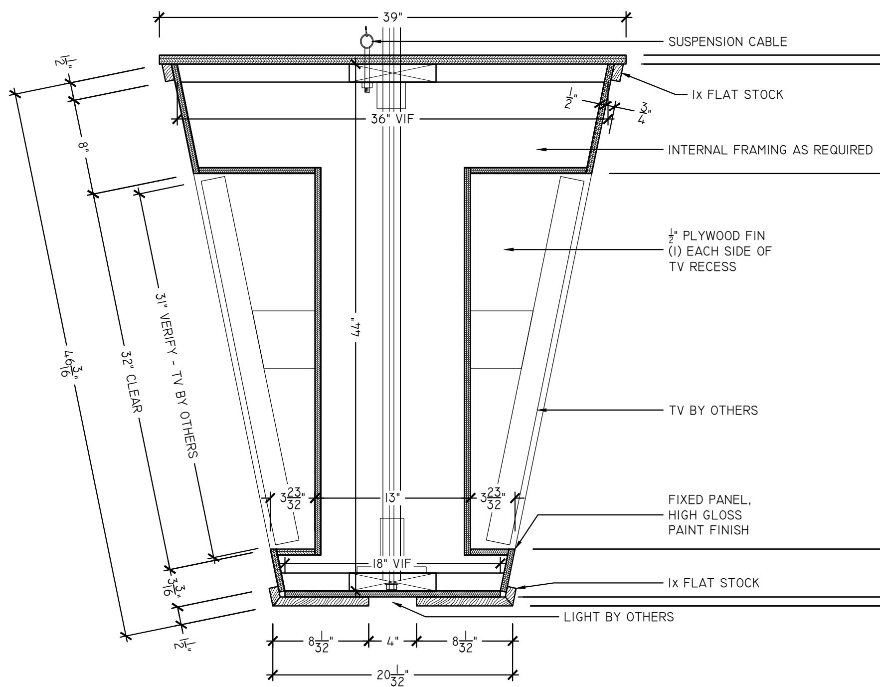
S2 SUSPENDED TV CANOPY - SECTION SCALE: 6" = 1'-0" ARCH REF: 9/A-904
