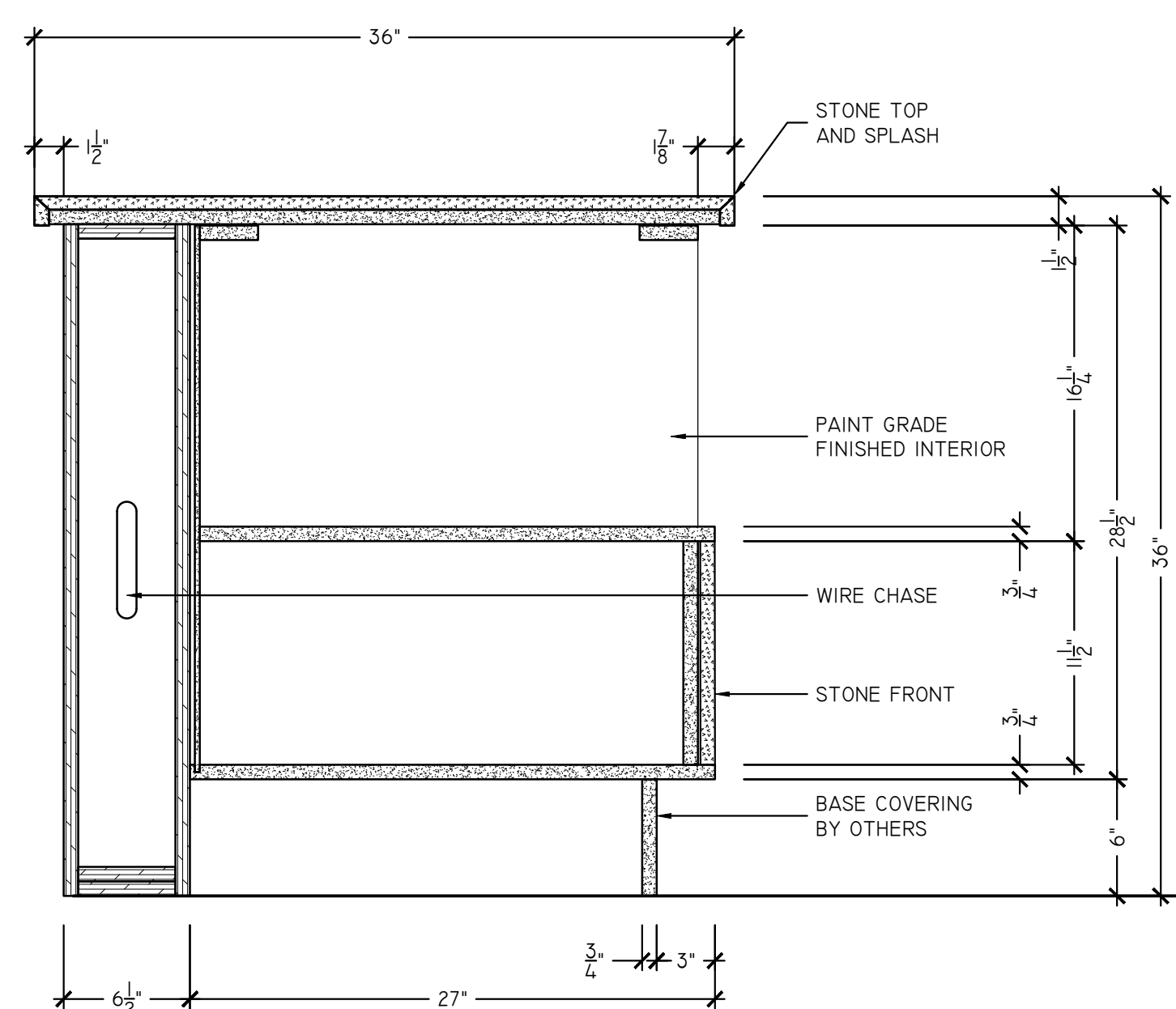
S2 BUFFET III - SECTION SCALE: 1-1/2" = 1'-0" ARCH REF: 6/1101
