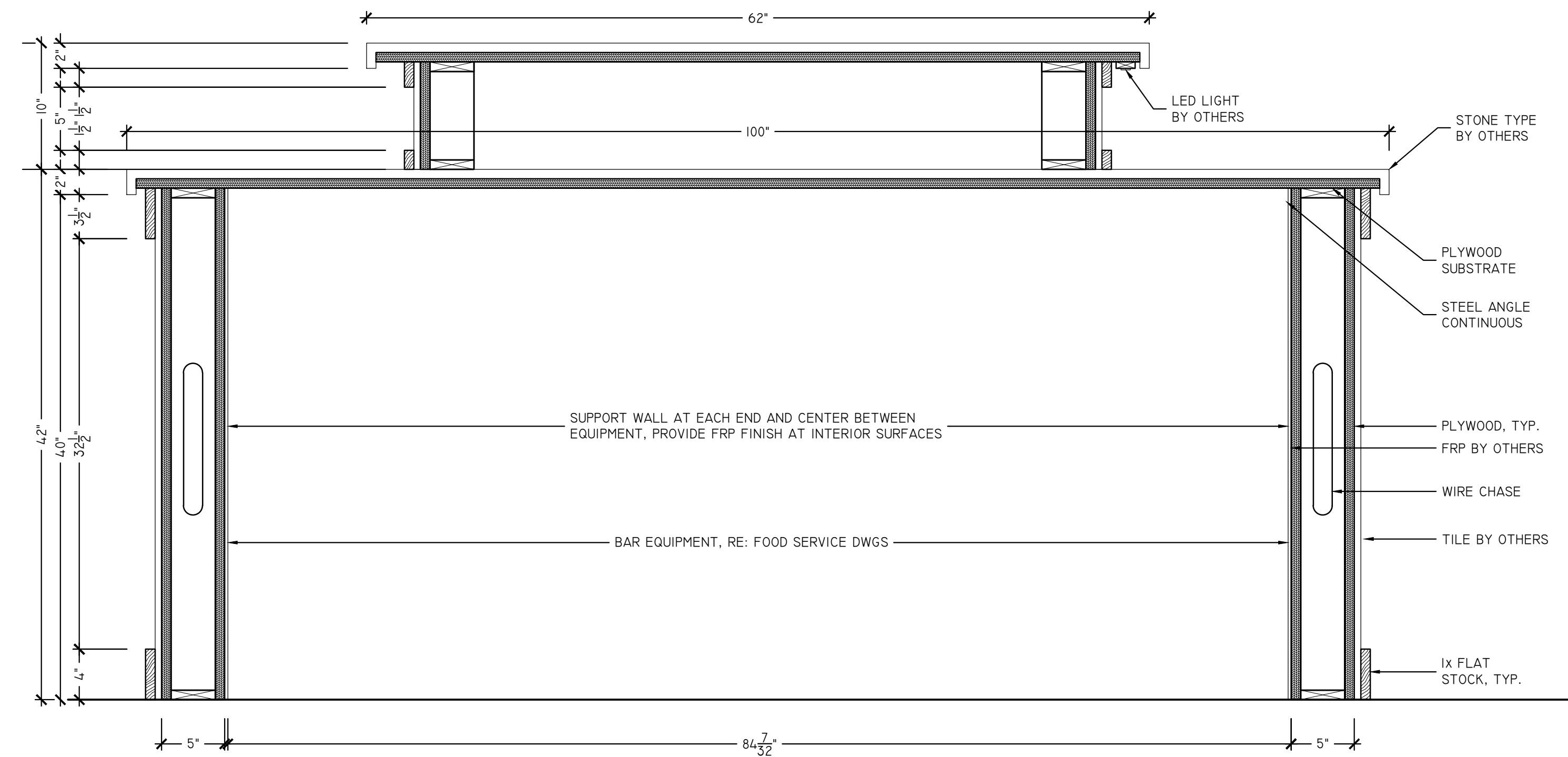
S3 INNER ISLAND - SECTION SCALE: 1-1/2" = 1'-0" ARCH REF: 3/1-401
