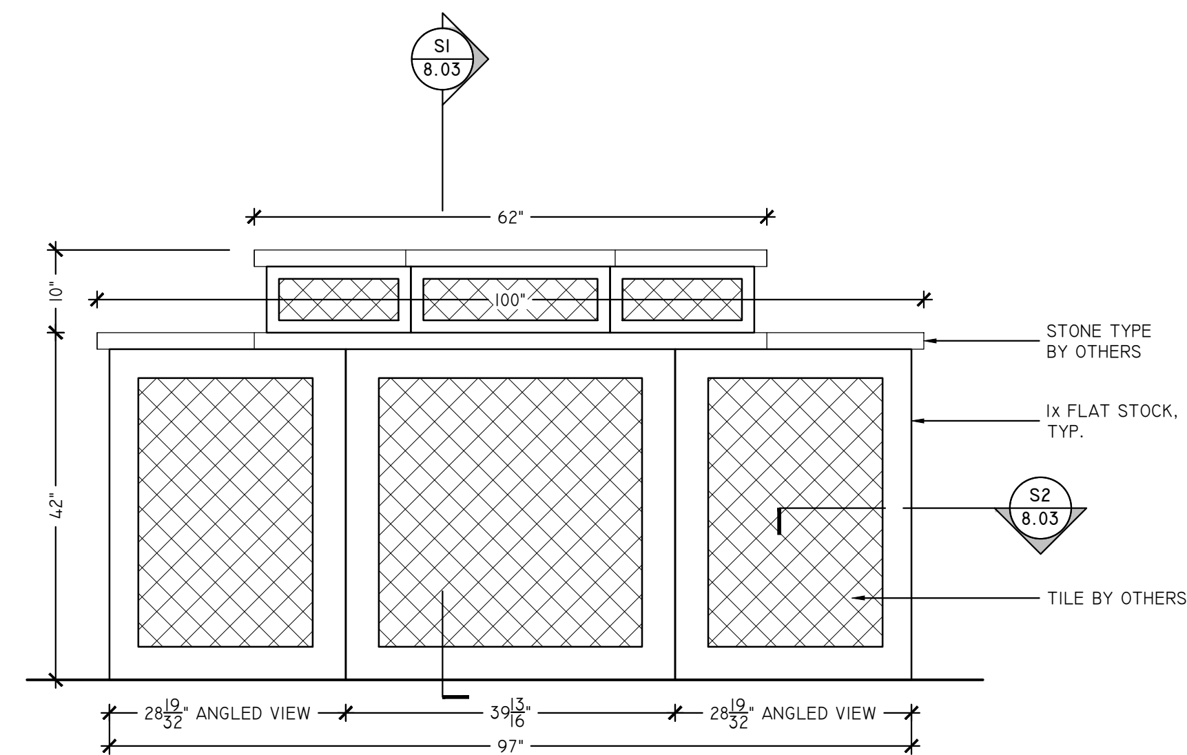
C INNER ISLAND - ELEVATION SCALE: 3/4" = 1'-0" ARCH REF: N/A
