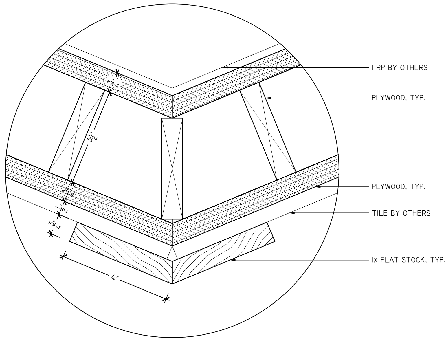
S2 MAIN BAR - SECTION SCALE: 1-1/2" = 1'-0" ARCH REF: 1/1-401
