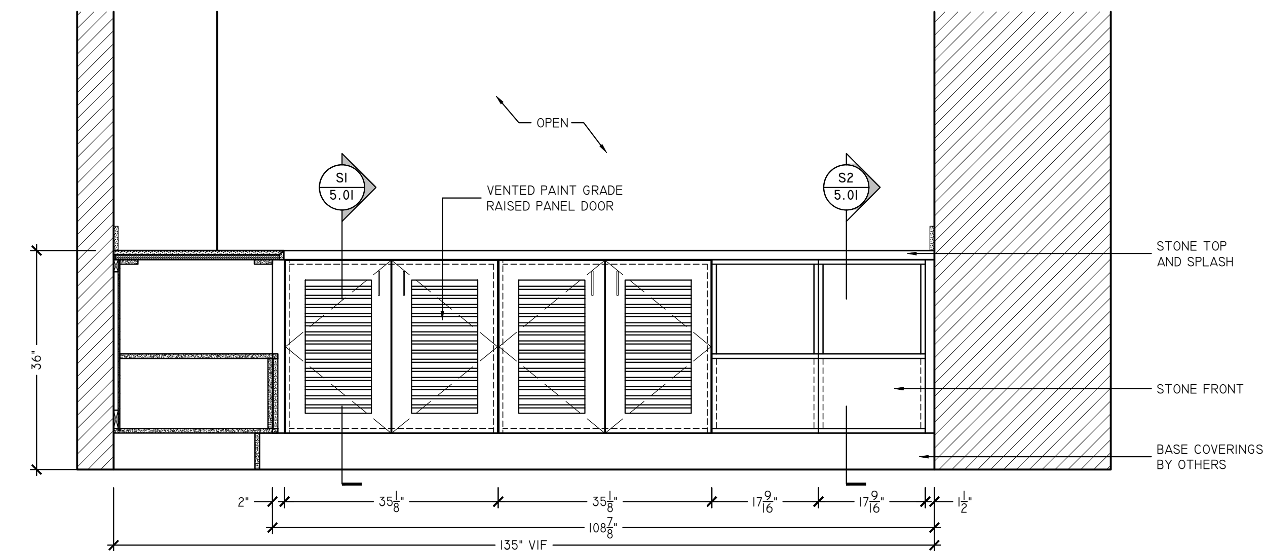
A BUFFET III - ELEVATION SCALE: 3/4" = 1'-0" ARCH REF: 6/1102
