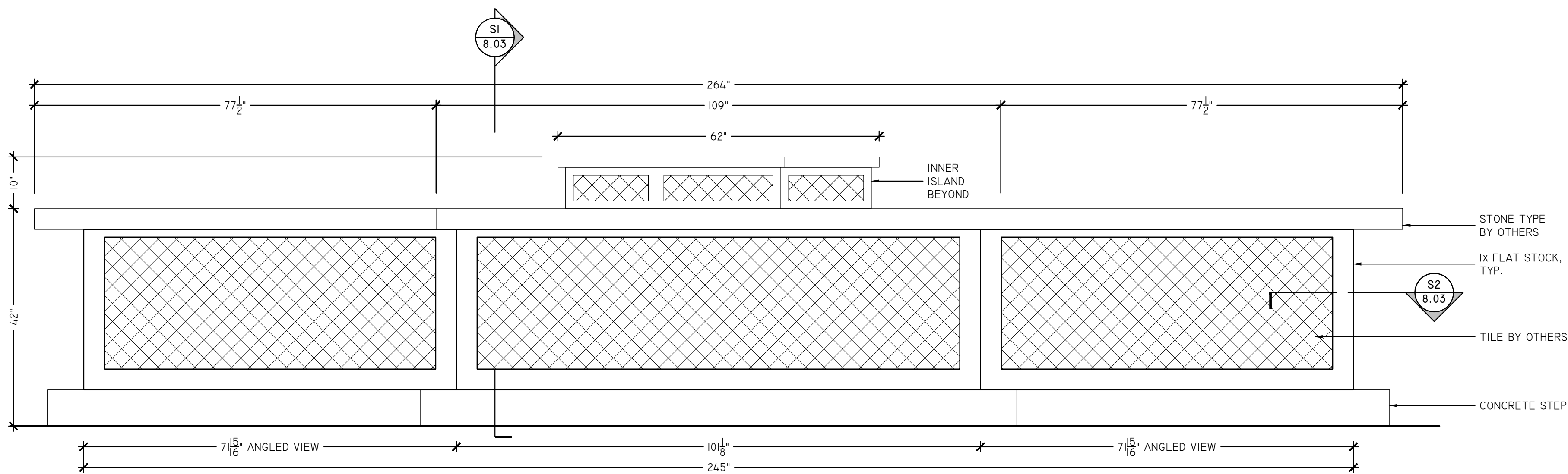
A MAIN BAR - ELEVATION SCALE: 3/4" = 1'-0" ARCH REF: 771-401
