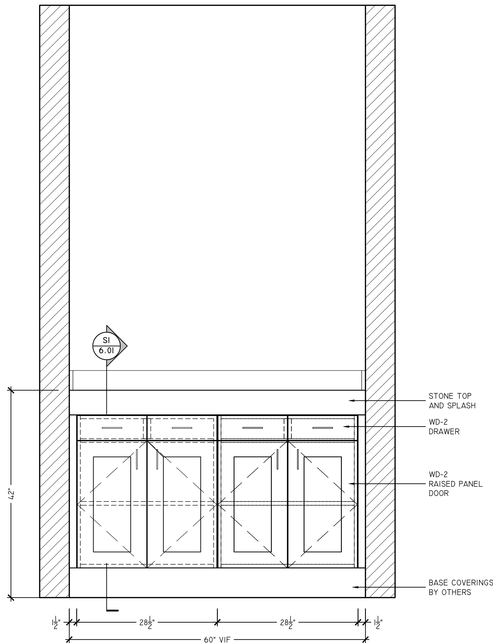
A SERVER STATION 103 - ELEVATION SCALE: 1" = 1'-0" ARCH REF: NONE
