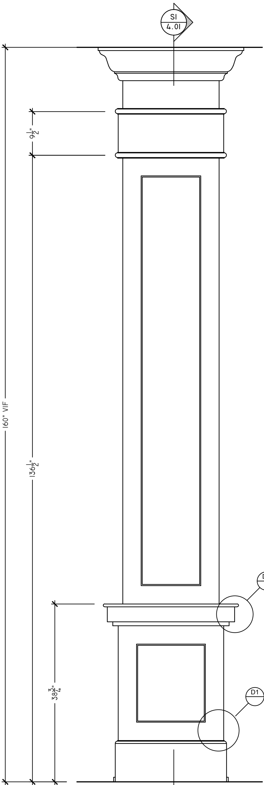
A TYPICAL COLUMN - ELEVATION SCALE: 1" = 1'-0" ARCH REF: 21/101
