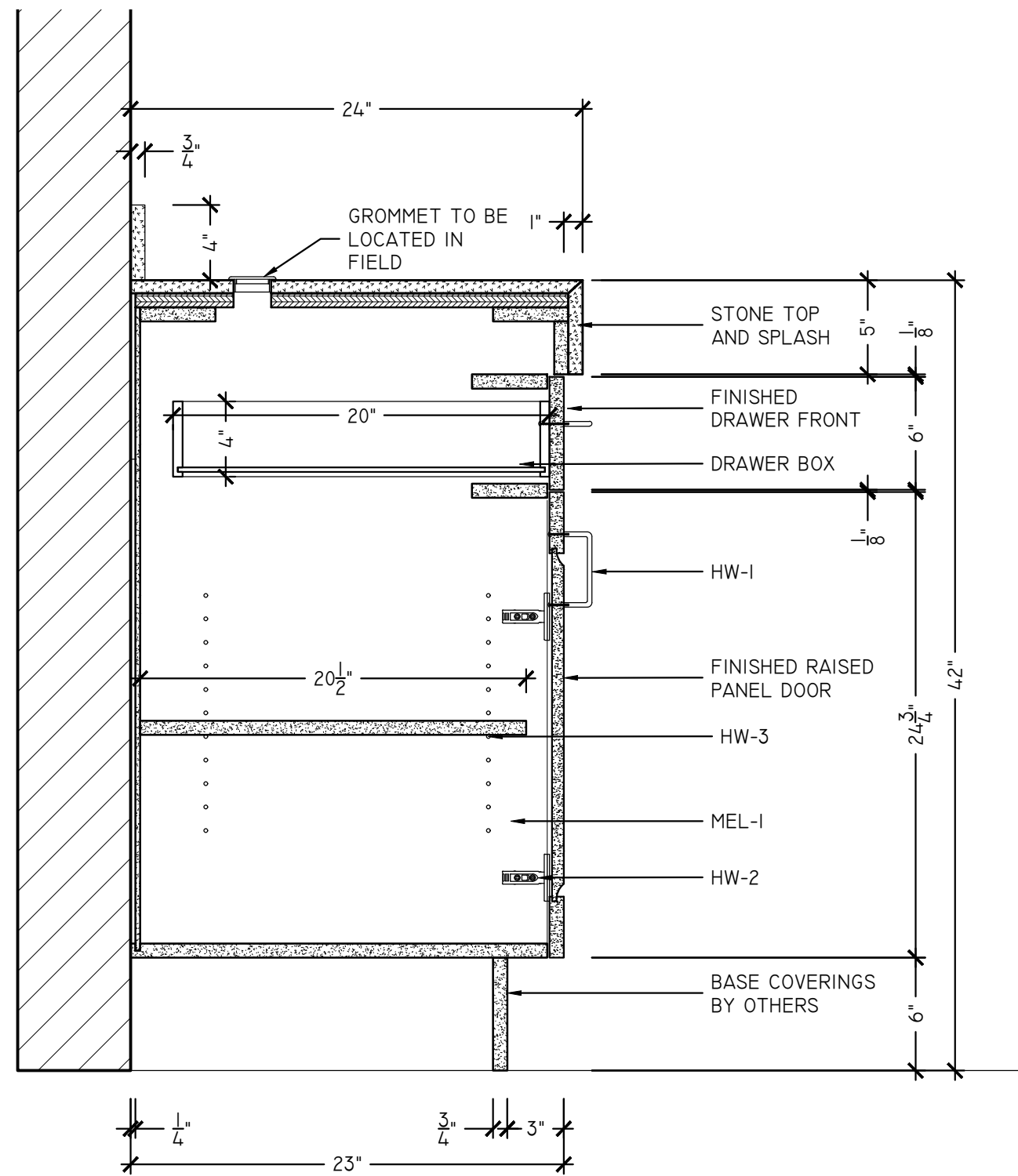
SI SERVER STATION 103 - SECTION SCALE: 1-1/2" = 1'-0" ARCH REF: 3/11.01
