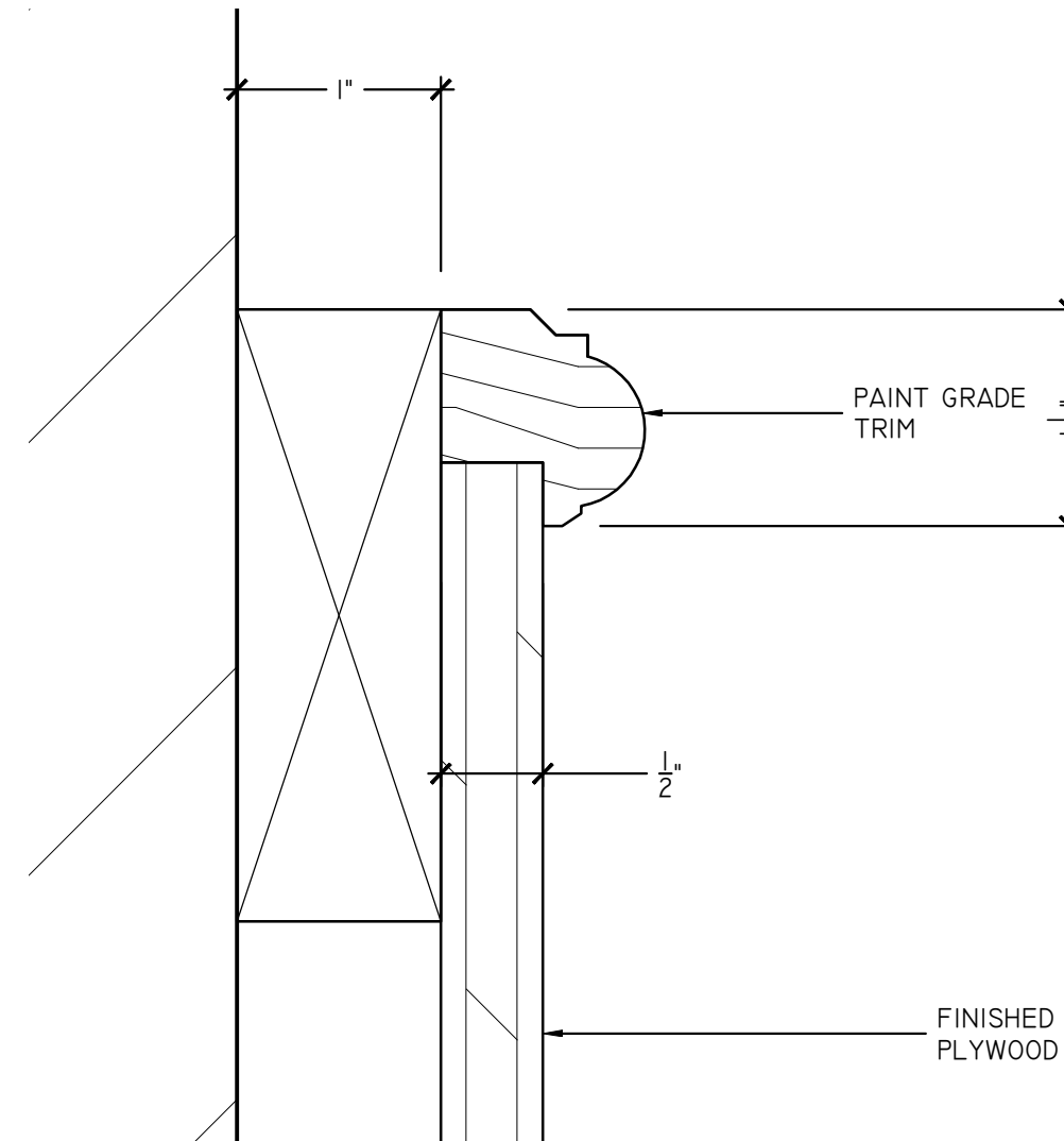
D5 TYPICAL COLUMN - DETAIL SCALE: 1'-0\"/>
