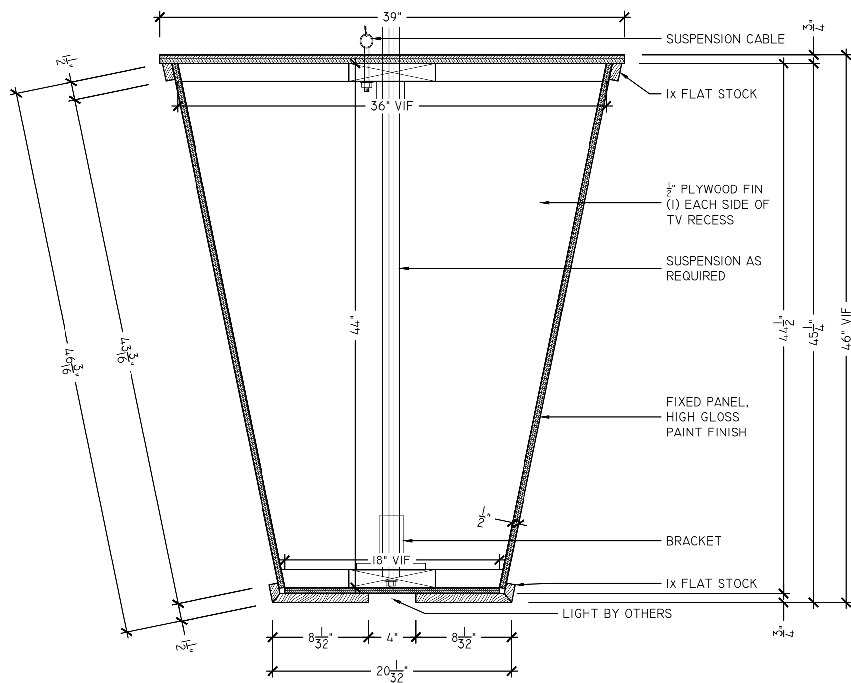
S1 SUSPENDED TV CANOPY - SECTION SCALE: 6" = 1'-0" ARCH REF: 13/A-904
