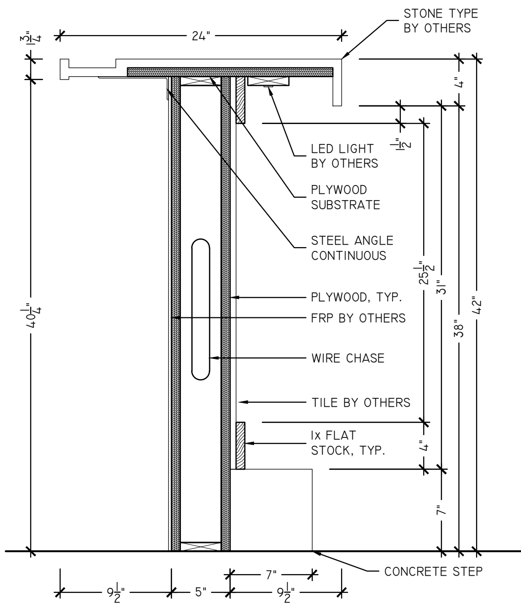
S1 MAIN BAR - SECTION SCALE: 1-1/2" = 1'-0" ARCH REF: 1/1-401
