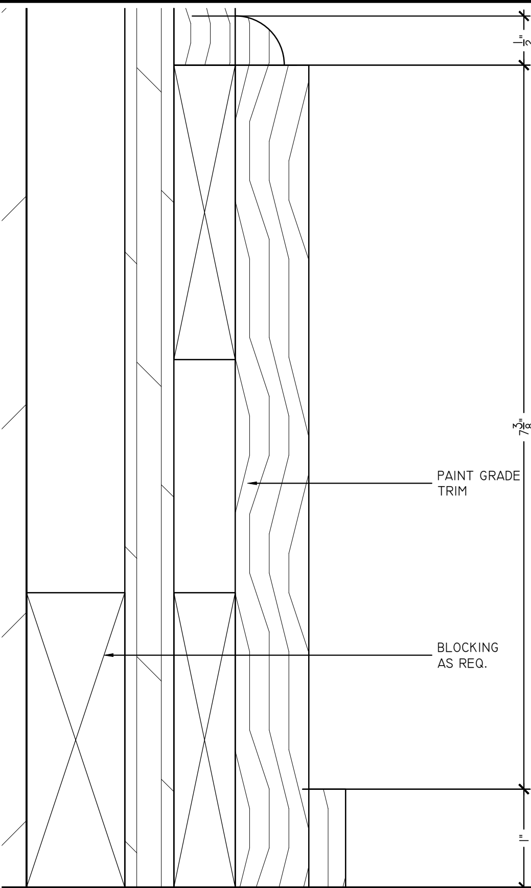
D3 TYPICAL COLUMN - DETAIL SCALE: 1'-0\"/>
