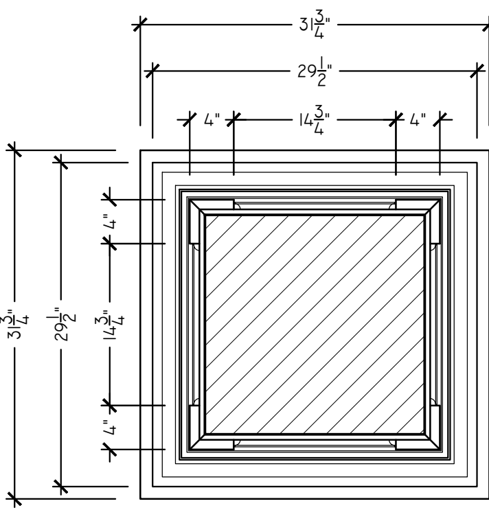
I TYPICAL COLUMN - PLAN SCALE: 1" = 1'-0" ARCH REF: 11/101
