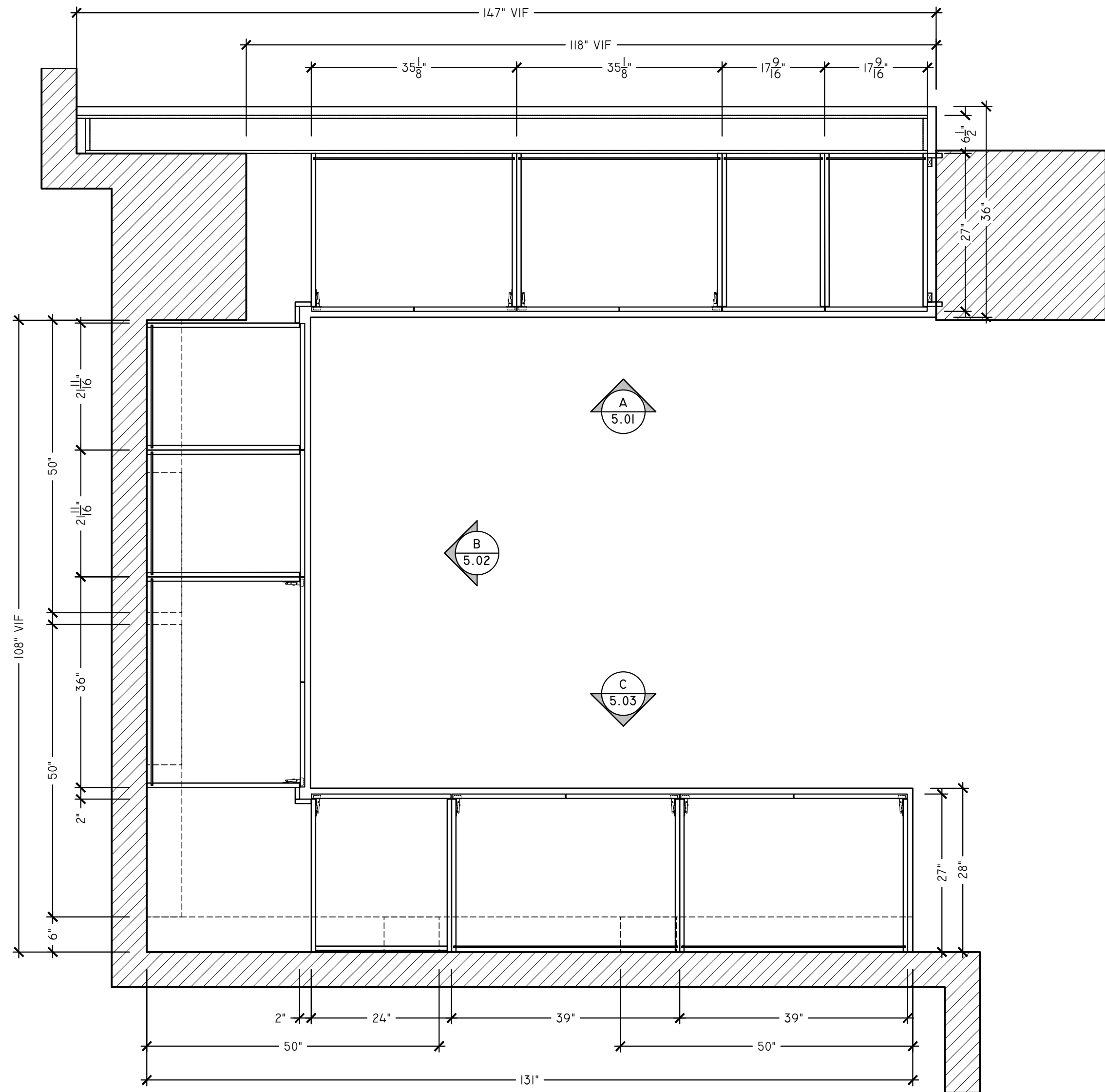
1 BUFFET III - PLAN SCALE: 3/4" = 1'-0" ARCH REF: 6/1101
